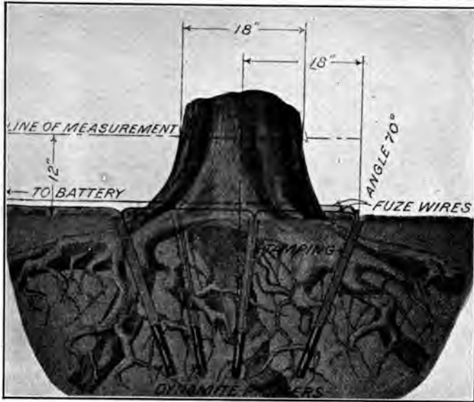
Fig. 22. Position of Charges for Large Stumps in Soft Ground
